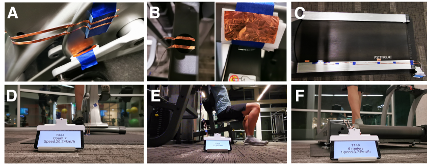
Fig. 11. Fitness tracking using FlexTouch . A and D: speed tracking on a cycling machine. B and E: push counter on a chest-press machine. C and F: distance and speed tracking on a treadmill.
