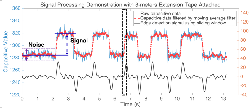
Fig. 3. Signal processing demo detecting the touch event.
